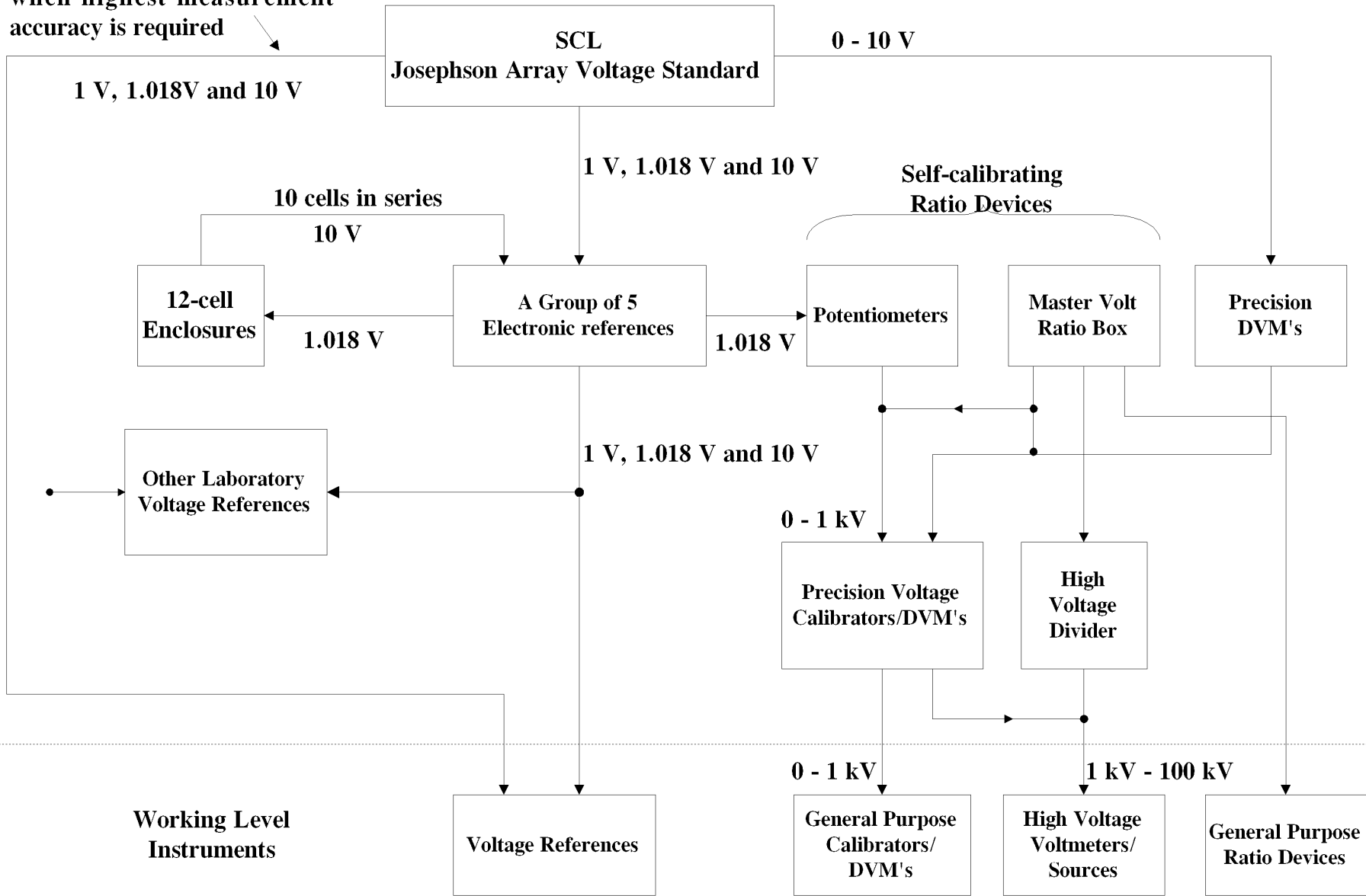
Traceability Chart : DC Voltage
