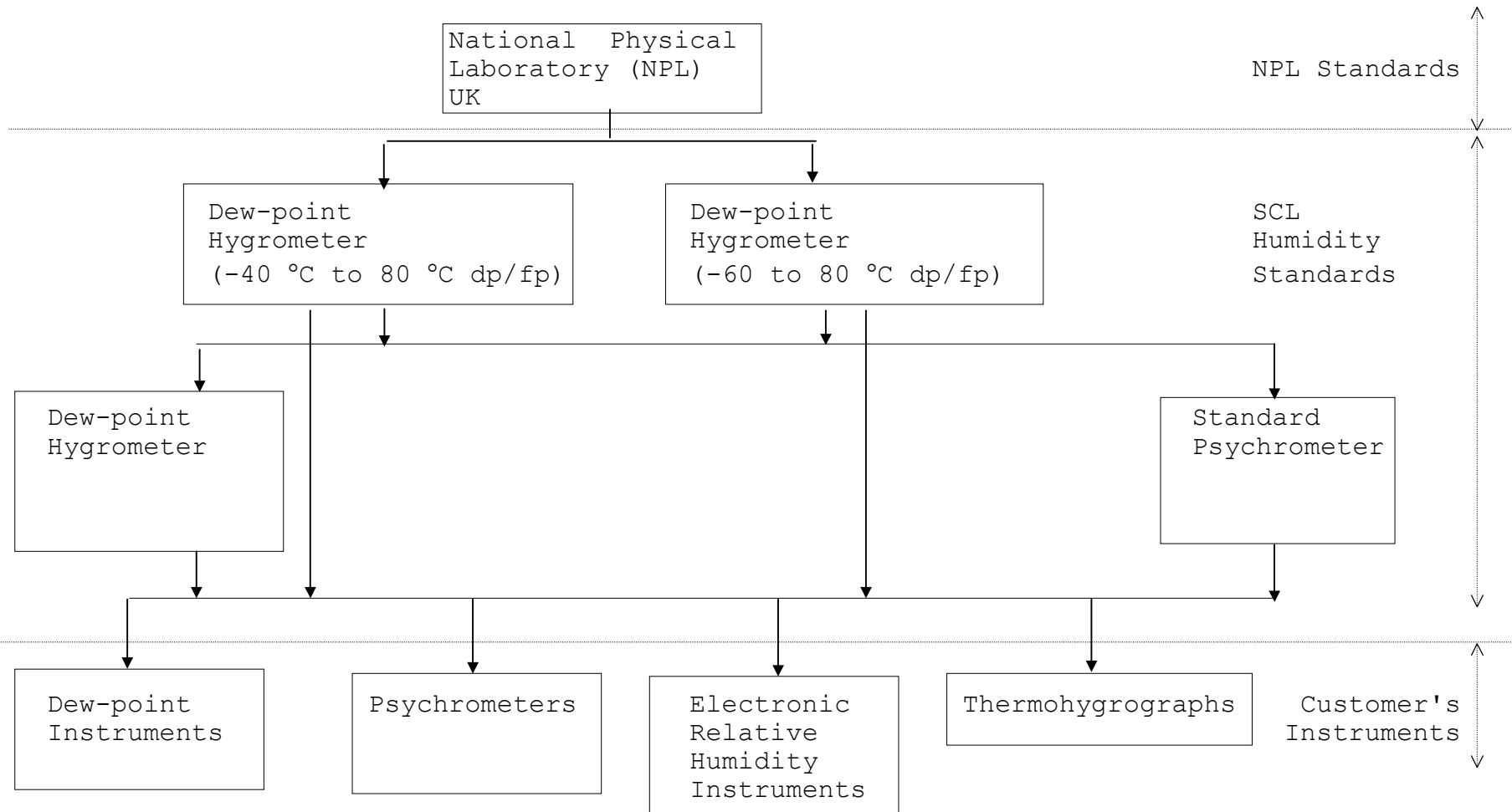
Traceability Chart for Humidity Measurement
