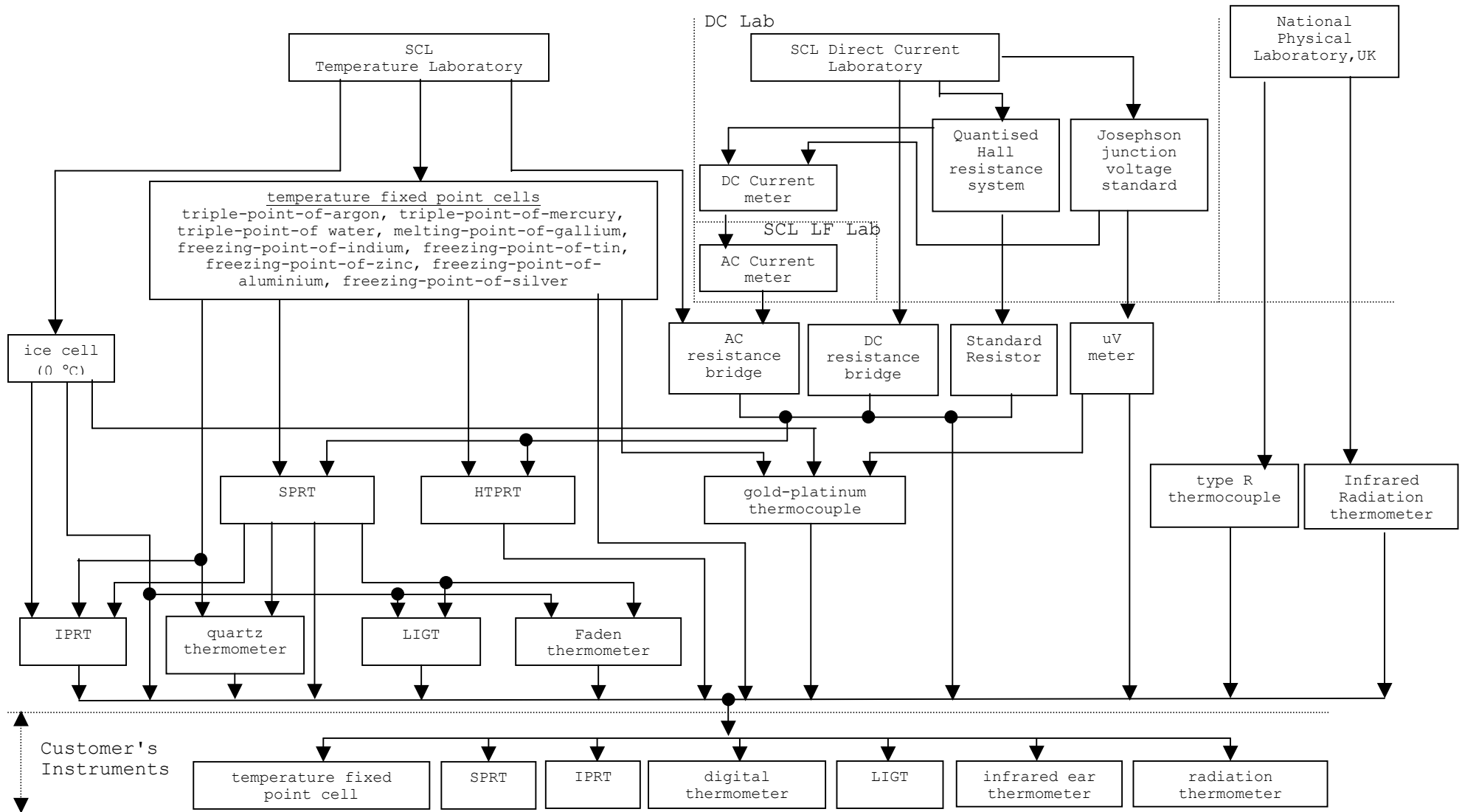
Traceability Chart for Temperature Measurement
